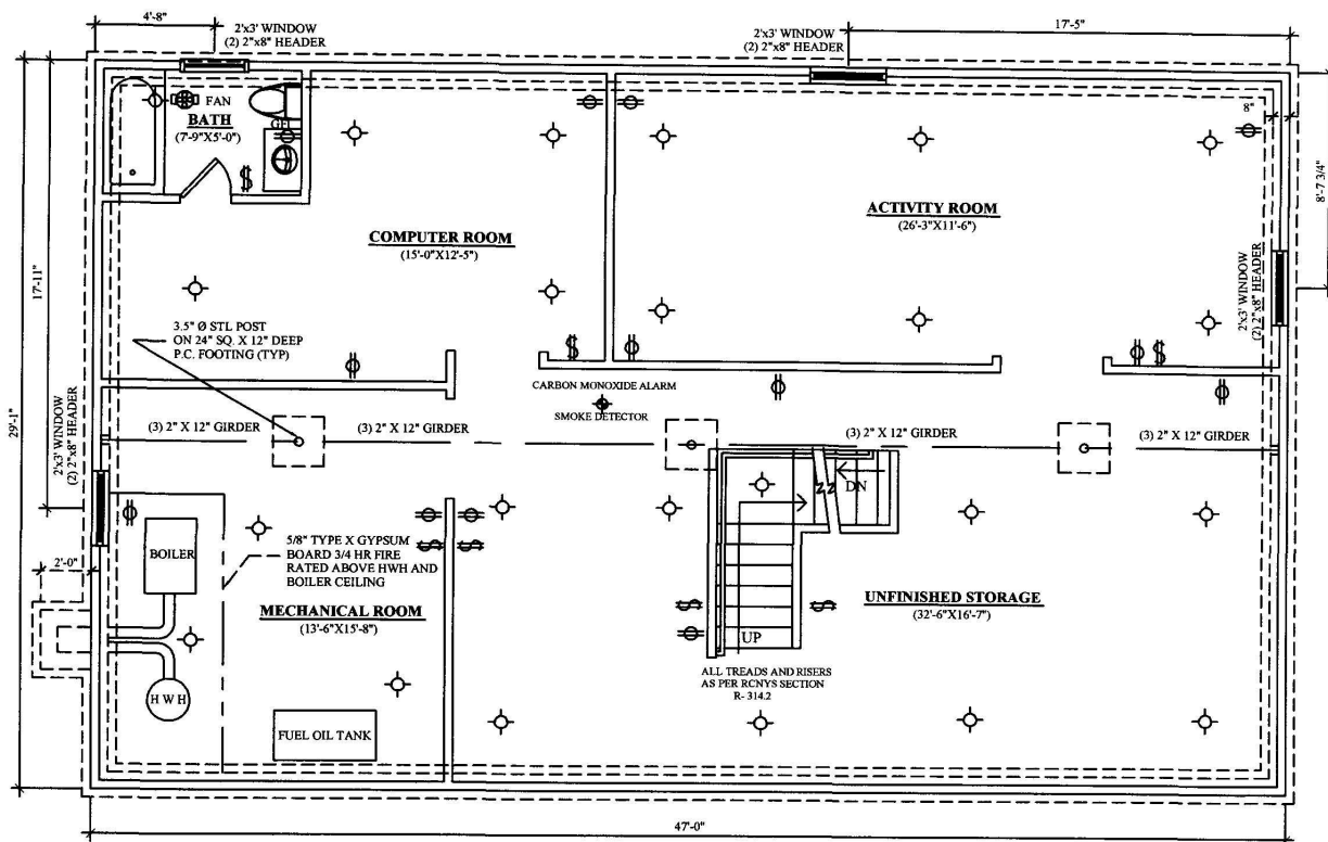
AS-BUILT BASEMENT PLAN
